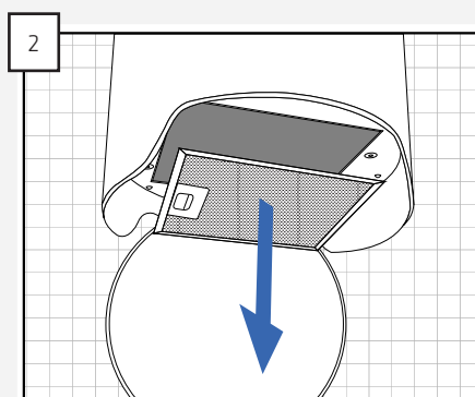
Remove the grease filter by pulling on the filter locking mechanism.
